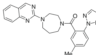
1 OX 1 R K i = 1.2 nM OX 2 R K i = 0.6 nM
