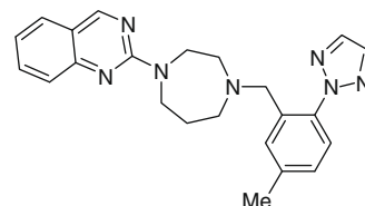
4 \text{OX}_1\text{R} K_i = 930 nM \text{OX}_2\text{R} K_i = 240 nM
