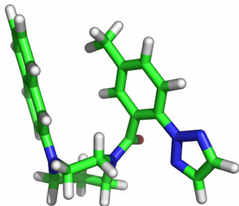
Figure 3. Predominant, low-energy structure of 2 using the MMFFs forcefield in chloroform at a constant dielectric constant of 4. The structure is consistent with the ^1\text{H} NMR for 2-rotamer A , and has a centroid separation distance of 5.2 Å.
