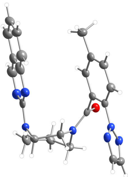
Figure 4. X-ray crystal structure of 1 illustrating the twist-boat conformation of the central diazepan ring, as well as the overall U-shaped structure present in the solid state.
