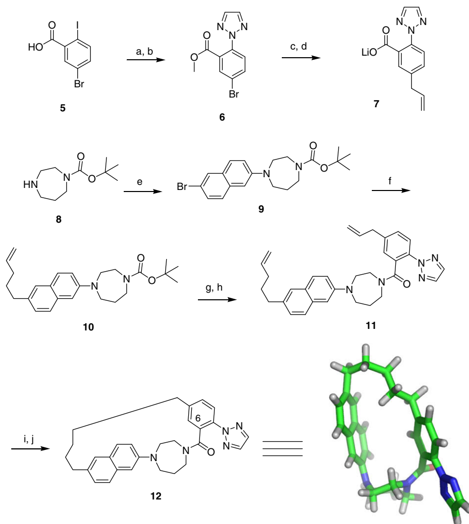
Scheme 1. Synthesis of the macrocycle. Reagents and conditions: (a) 1H-1,2,3-triazole, CuI, K 3 PO 4 , DMF, 60 °C; (b) HCl(g), MeOH (36% for two steps); (c) tetraallyllytin, tetrakis(triphenylphosphine) Pd(0), LiCl, DMF, 125 °C (83%); (d) LiOH, THF/MeOH/H 2 O, 45 °C (quant.); (e) 2,6-dibromonaphthalene, NaO t Bu, BINAP, Pd 2 (dba) 3 , PhMe, 100 °C (46%); (f) 4-pentenylzinc bromide, Pd(PtBu 3 ) 2 , THF, 75 °C (38%); (g) HCl, Et 2 O; (h) 7 , EDC, HOBT, TEA, DMF, 50 °C (63% for two steps); (i) Zhan 1B, DCE, 40 °C (12%); (j) H 2 , Pd/C, EtOAc (87%).
