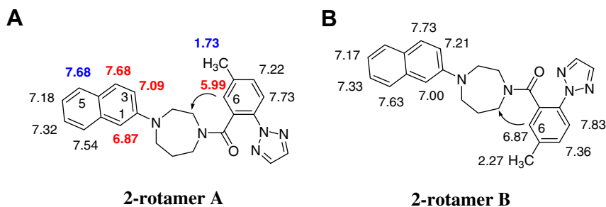
Figure 2. Panel A: ^1\text{H} NMR data for the major rotamer of compound 2 , 2-rotamer A , determined by analysis of 2 at 25^\circ\text{C} in \text{CD}_3\text{OD} . The NOE used to assign the amide rotamer is indicated by a black arrow, and the NOE's used to establish the U-shaped conformation are illustrated by the proton resonance assignments (in ppm) highlighted in red and blue. Panel B: similar data as presented in Panel A, but for the minor rotamer, 2-rotamer B . Rotamer A accounts for 58% of the solution and rotamer B is 42%.
