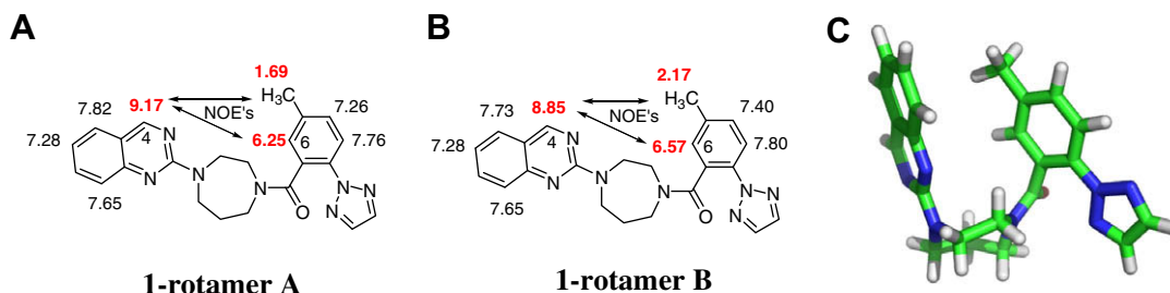
Figure 1. Panel A: ^1\text{H} NMR data for the most highly populated rotamer of compound 1 , 1-rotamer A , determined by analysis of 1 at -40^\circ\text{C} in \text{CD}_3\text{OD} . Key NOE correlations are indicated by black arrows, and proton resonance assignments (in ppm) are illustrated; resonances highlighted in red are most relevant for deducing solution conformation. Panel B: similar data as presented in Panel A, but for the second most populated rotamer, 1-rotamer B ( Rotamer A accounts for 45% of the solution and rotamer B is 36%). Panel C: a low-energy conformation computed for 1 that is consistent with the NMR data. 5
