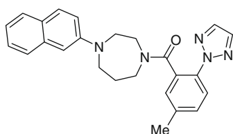
2 OX 1 R K i = 2 nM OX 2 R K i = 2 nM
