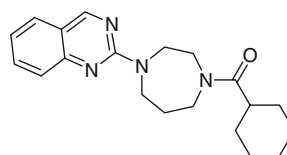
3 \text{OX}_1\text{R} K_i = 9,800 nM \text{OX}_2\text{R} K_i = 550 nM
